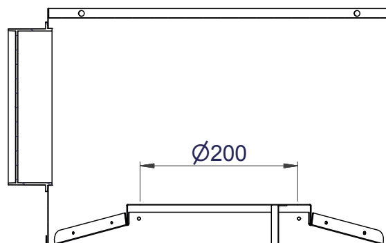
A-A (1/5)
